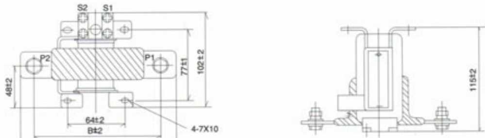
LQG2-0.5(150~1000/5A)
