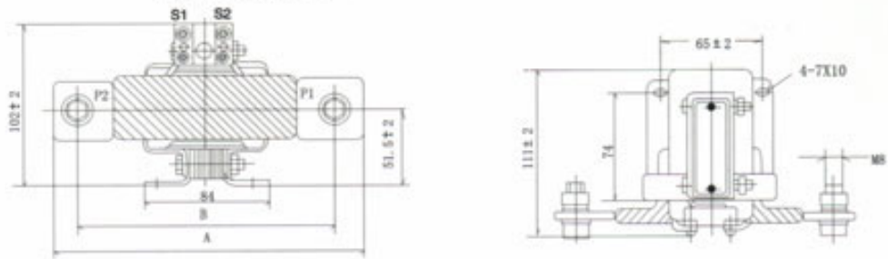
LQG-0.5(5-100/5)
