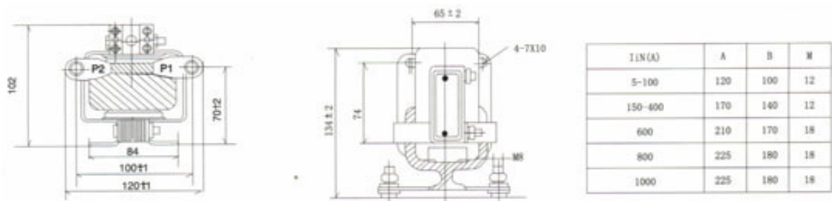
LQG-0.5(5-100/5)
