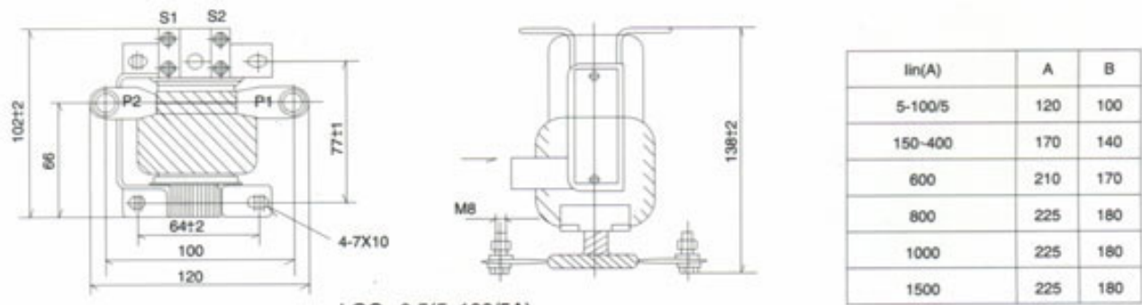
LQG2-0.5(5-100/5A)
